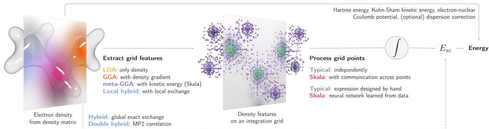
(a) Anatomy of an exchange-correlation functional
